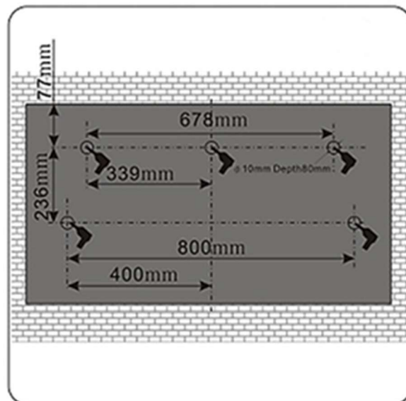
Rear fixing mounting template:
